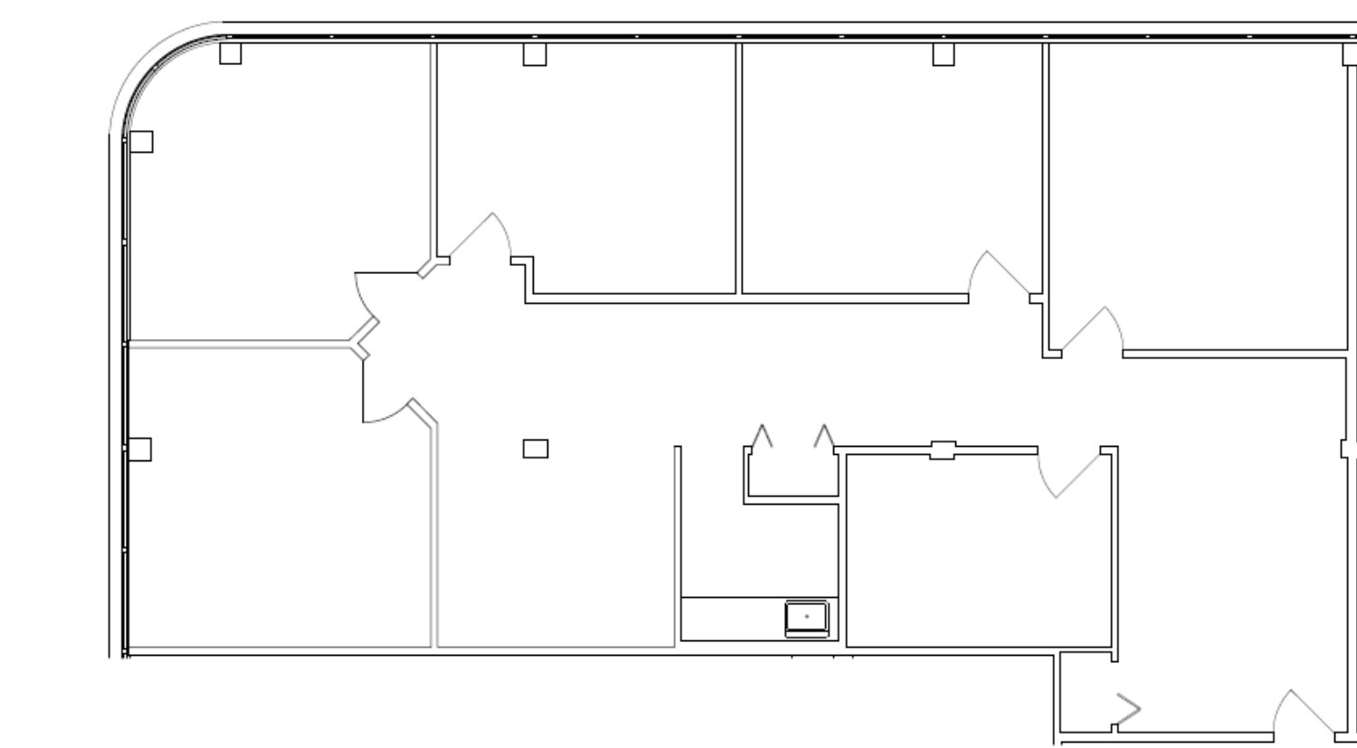
KEY PLAN
